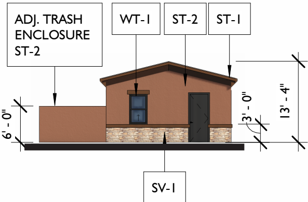
13 | SOUTHEAST ELEVATION
