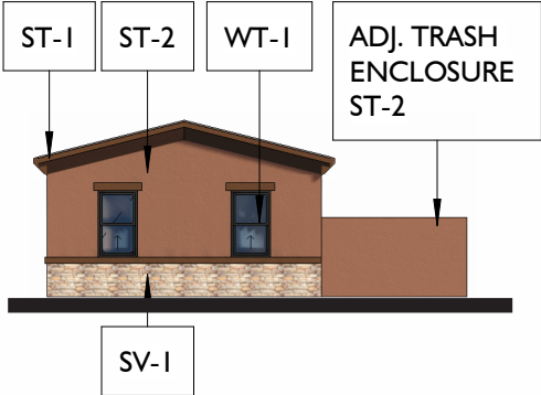
11 | NORTHEAST ELEVATION
