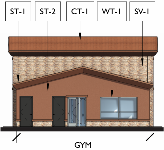
8 | SOUTHEAST ELEVATION
