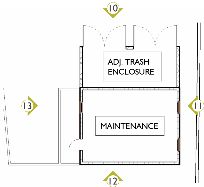
9 | MAINTENANCE FLOOR PLAN
