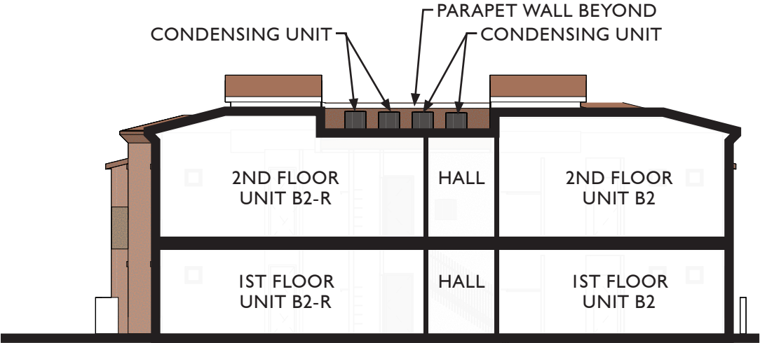
TYPICAL BUILDING B SECTION
