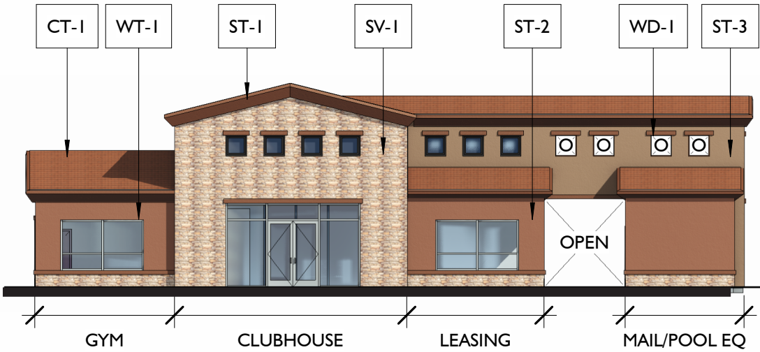
7 | SOUTHWEST ELEVATION
